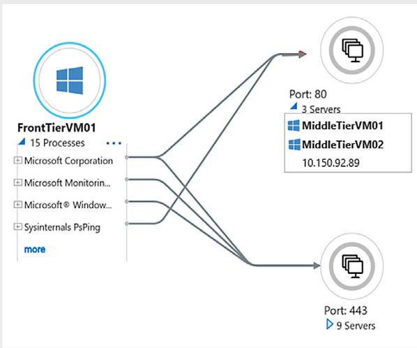
Figure 4. Visualise dependencies
